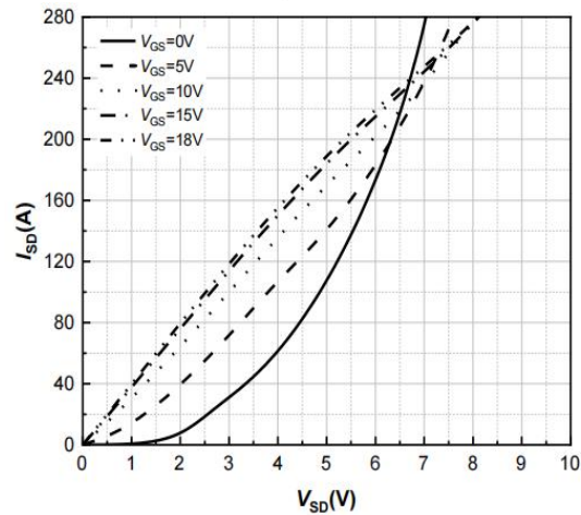
Figure 13. 3rd Quadrant Characteristic T_j = -40^\circ\text{C}
